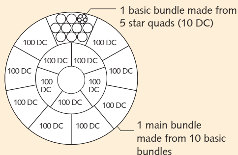
Structure of a 1500-paired cable comprising 15 main bundles of 100 DC
