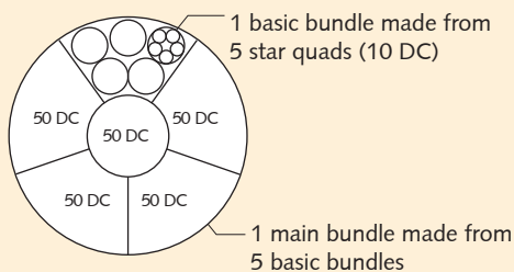
Structure of a 300-paired cable comprising 6 main bundles of 50 DC
