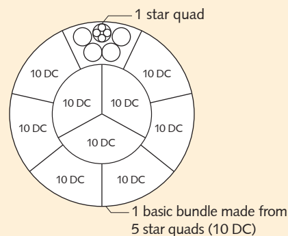
Comprising 10 basic bundles = 100 DC
