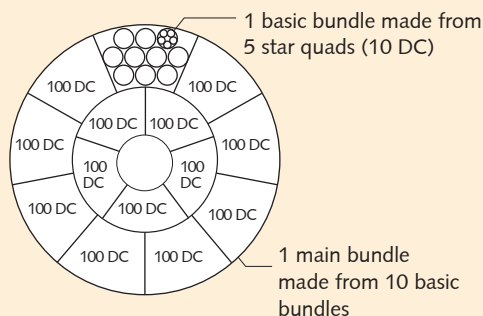
Structure of a 1500-paired cable comprising 15 main bundles of 100 DC
